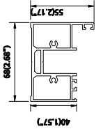
Top Track
